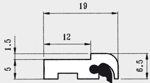
RASCHIATORE WIPER Mod. 008/32447 Materiale Ottone-Poliuretano Material Brass-Polyurethane In barre / Bars Length 3000 mm
