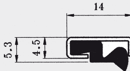
RASCHIATORE WIPER Mod. 008/40295 Materiale Acciaio-Poliuretano Material Steel-Polyurethane In barre / Bars Length 560 mm
