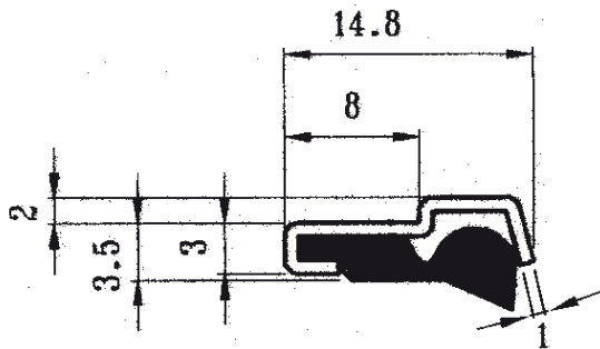
RASCHIATORE WIPER Mod. 008/45700 Materiale Acciaio-Poliuretano Material Steel-Polyurethane In barre / Bars Length 3000 mm
