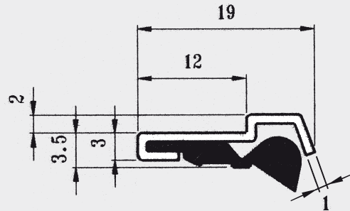
RASCHIATORE WIPER Mod. 008/11111 Materiale Acciaio-Poliuretano Material Steel-Polyurethane In barre / Bars Length 3000 mm
